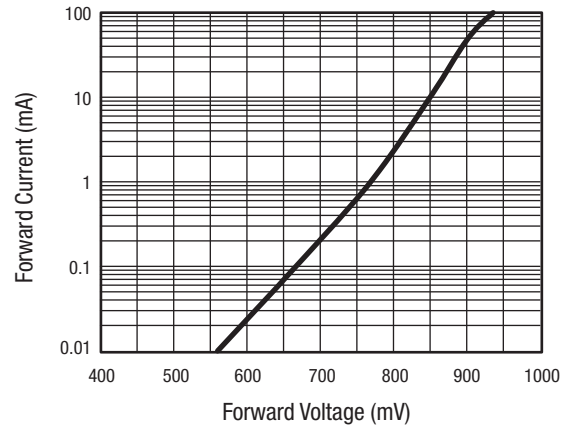
Figure 2. DC Characteristics
